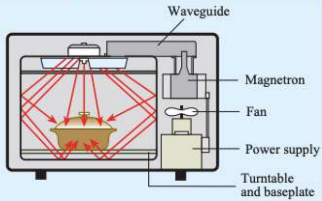
Figure 1. Schematic diagram of a typical microwave oven.
